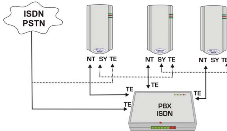
Figure 3-10 Usage of SY connector
