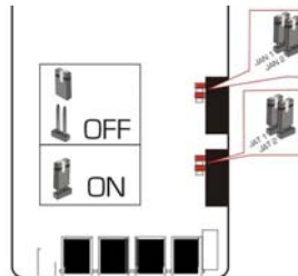
Figure 3-7 Location of JAT1, JAT2, JAN1 and JAN2 jumpers
