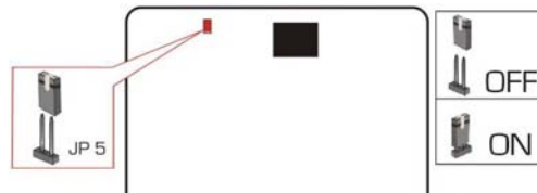
Figure 3-6 JP5 jumper location
